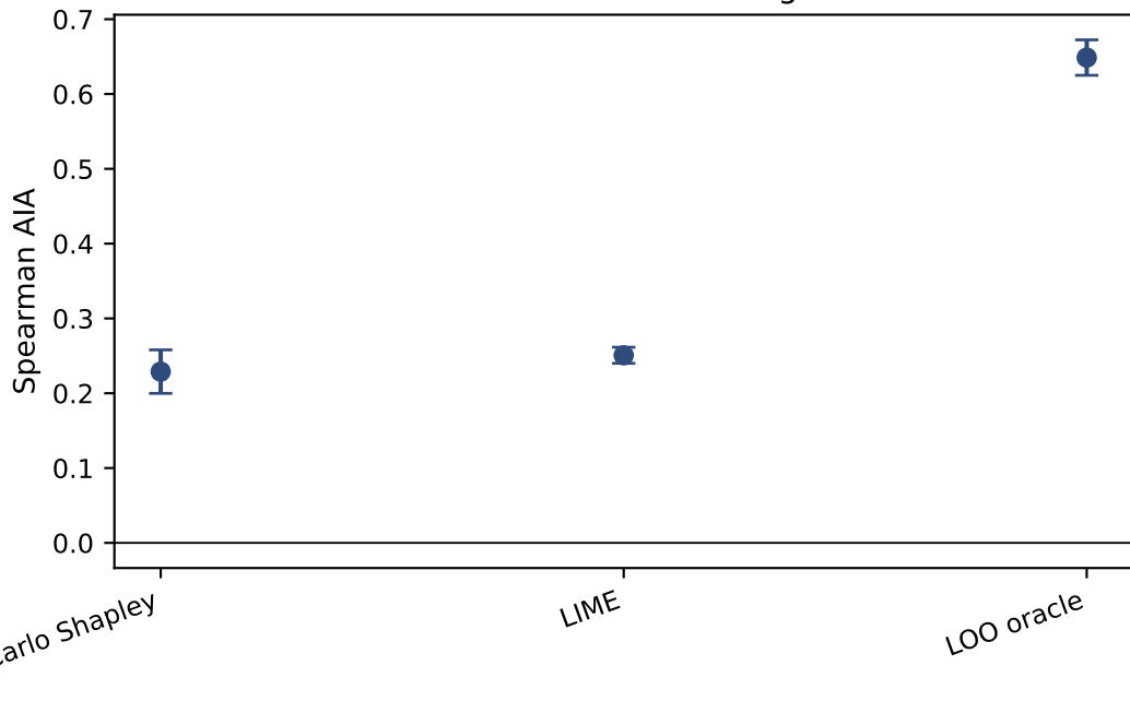
Attribution-Intervention Alignment
