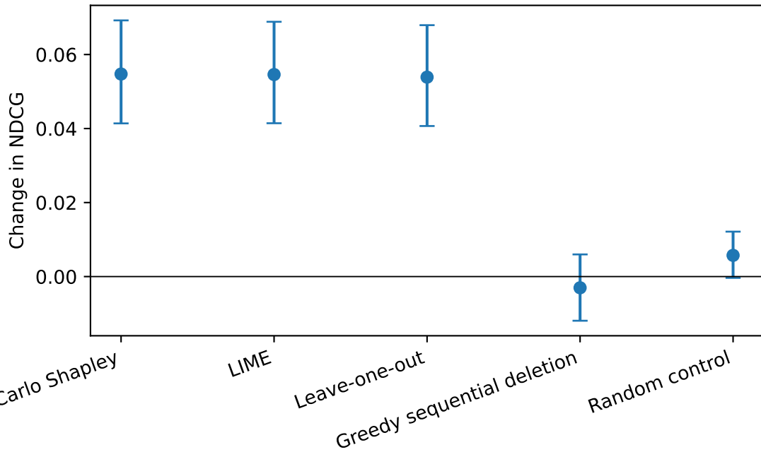
Realized NDCG effect of selected action
