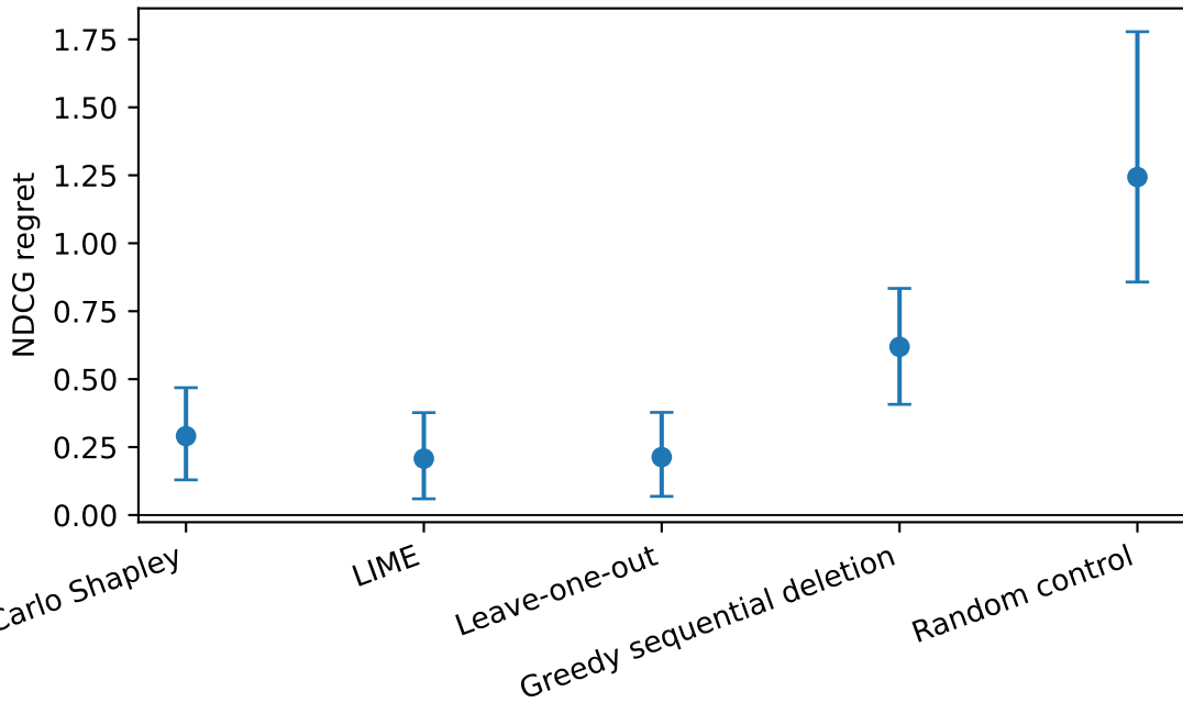
Normalized NDCG intervention regret
