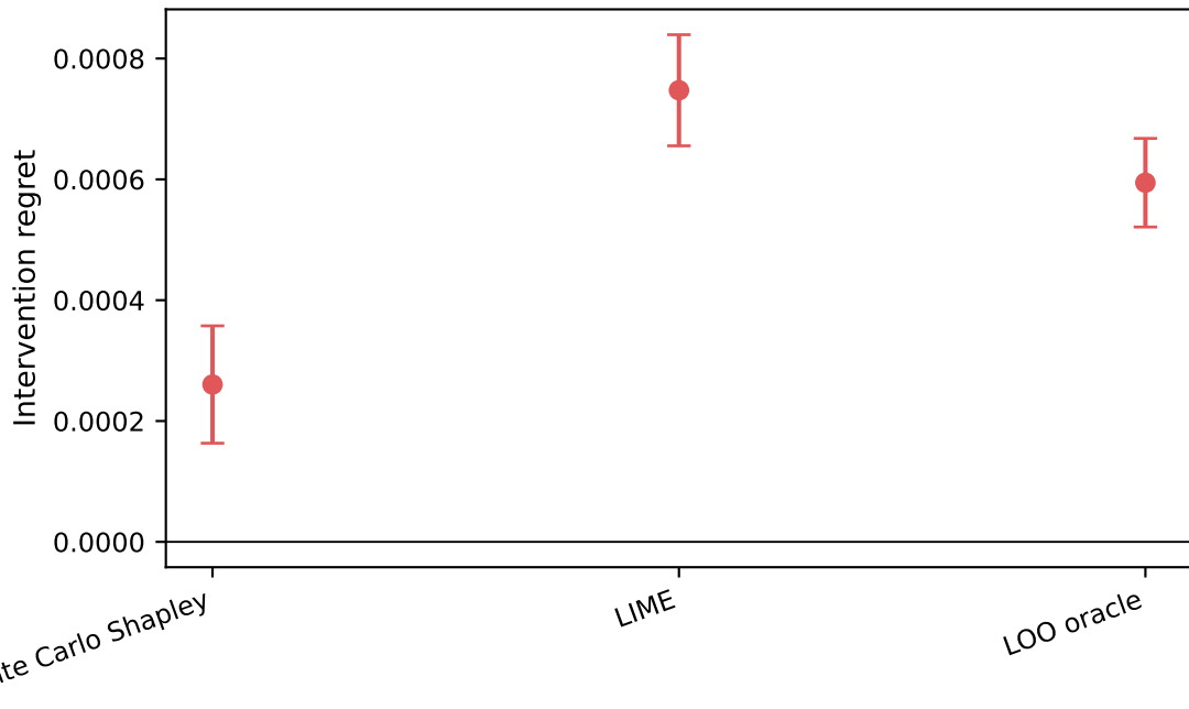
Joint intervention regret (B=2)
