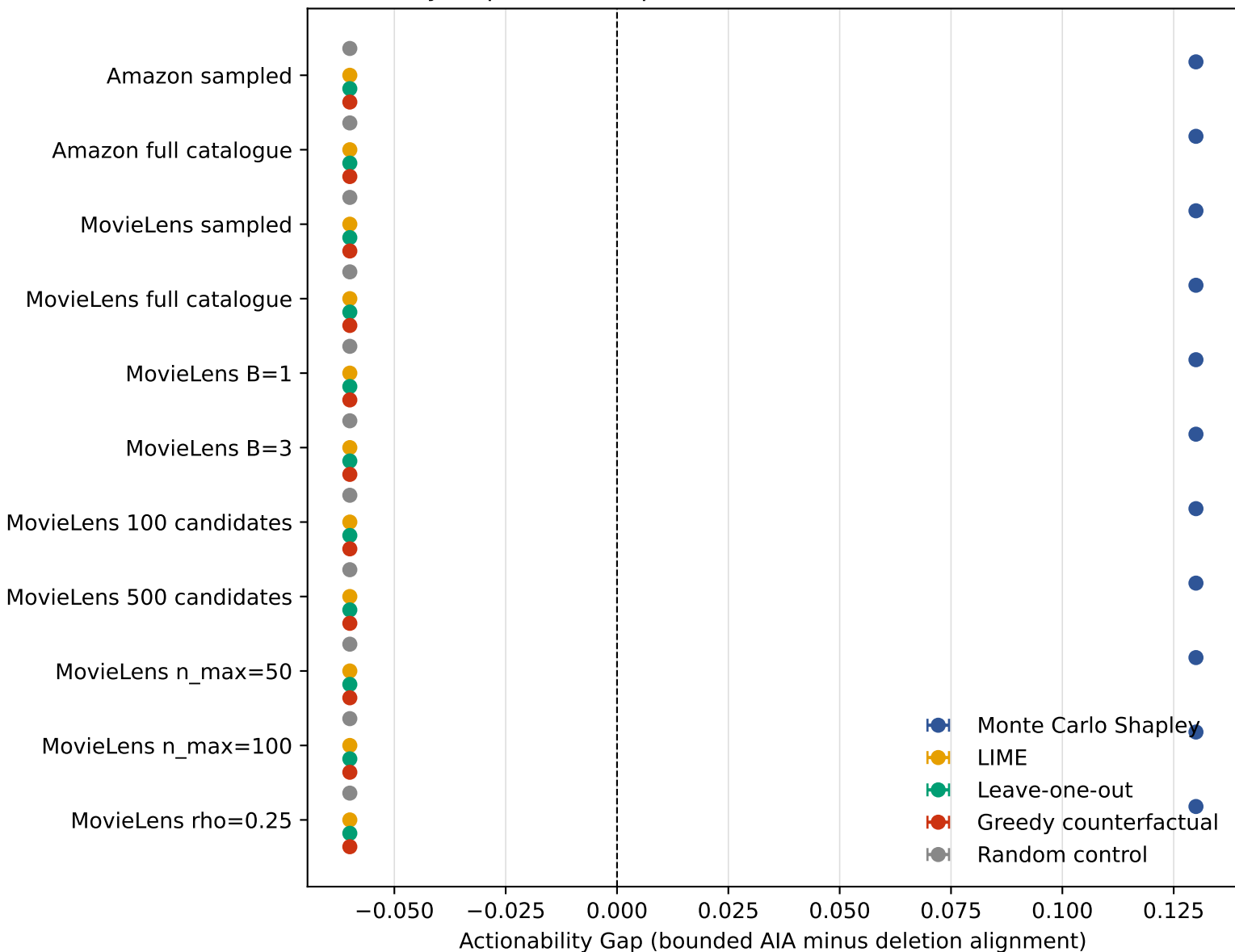
Actionability Gap across all predeclared ItemKNN conditions (all 5 methods)
