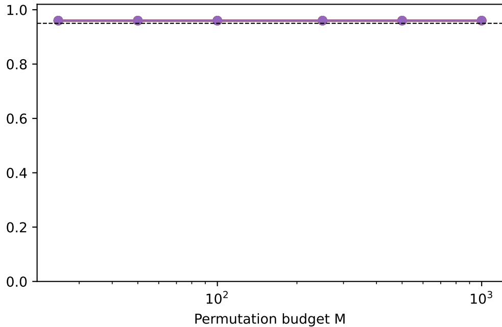
Rank convergence
