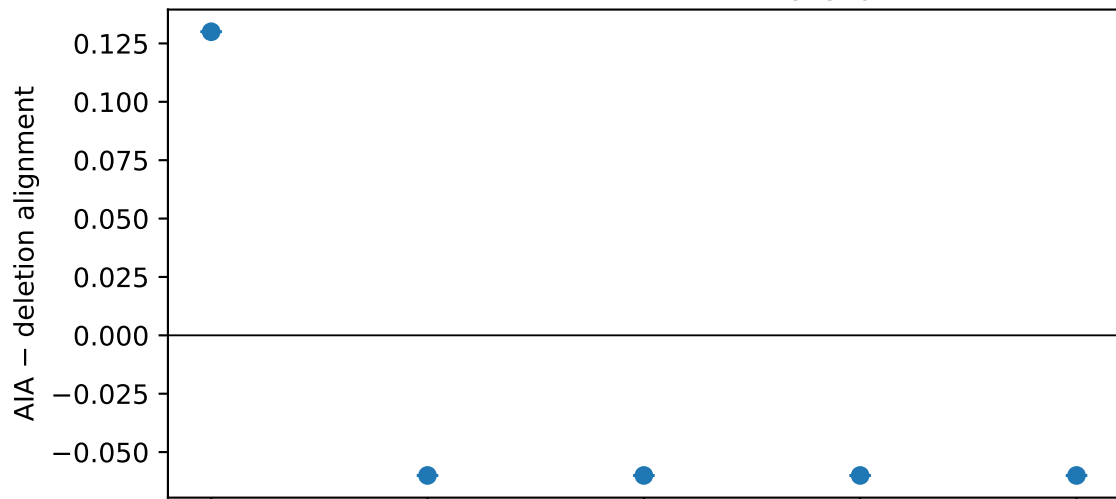
Faithfulness-actionability gap
