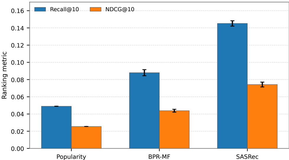
Fig. 5: External ranking robustness
