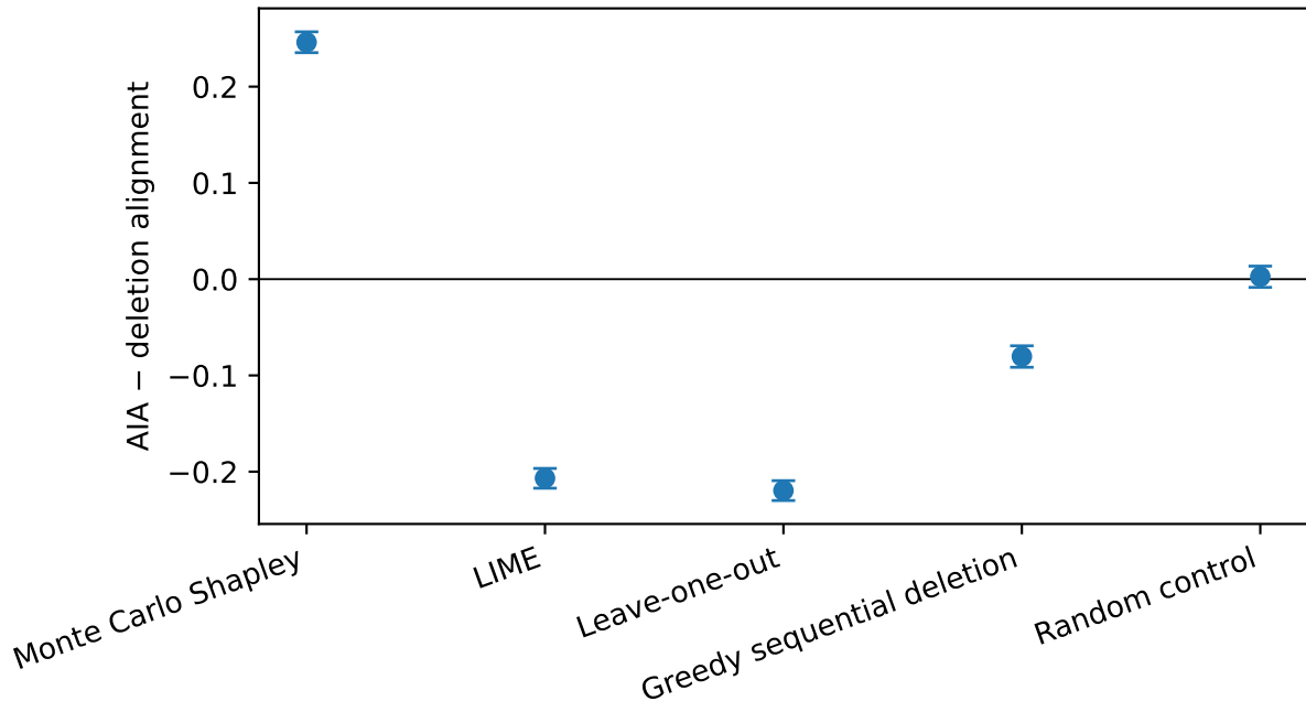
Faithfulness-actionability gap
