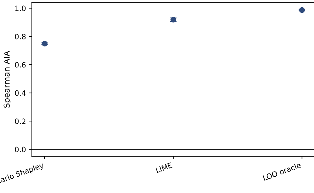
Attribution-Intervention Alignment
