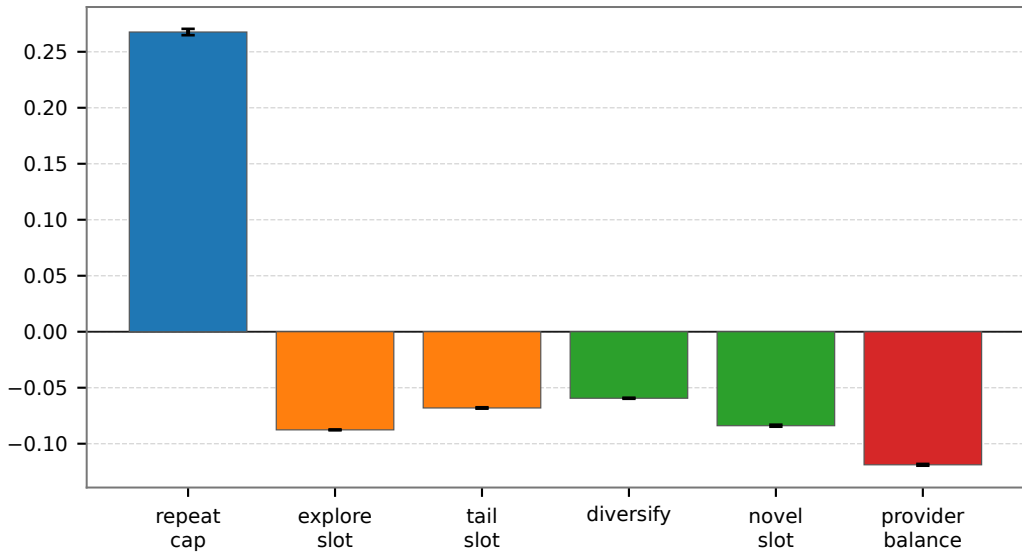
Fig. 2: Exact robust-game intervention attribution
