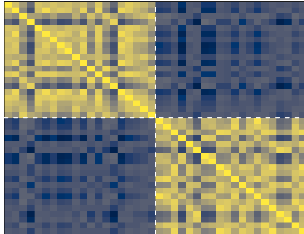
Riemannian Distance Matrix N \times N (Intra-group structure appears clearly)
