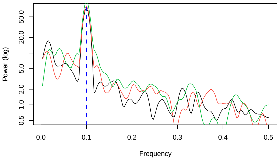
Daniell Smoothed Spectrum (Patient 1)
