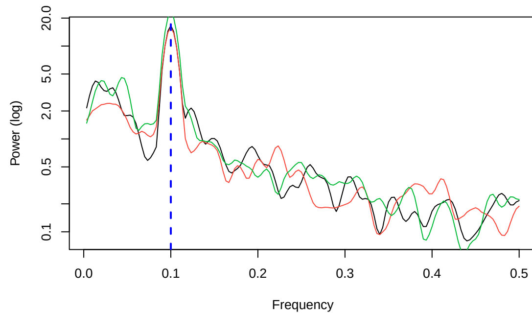
Daniell Smoothed Spectrum (Patient 21)
