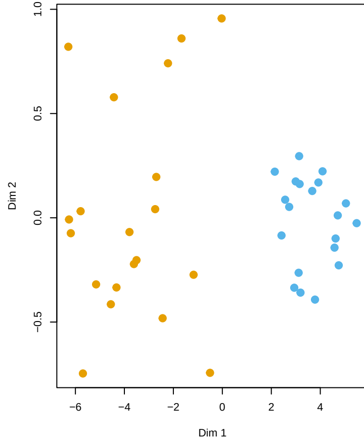
MDS – LERM (Model A)
