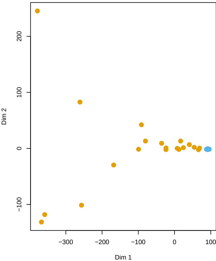
MDS – Euclidean (Model A)
