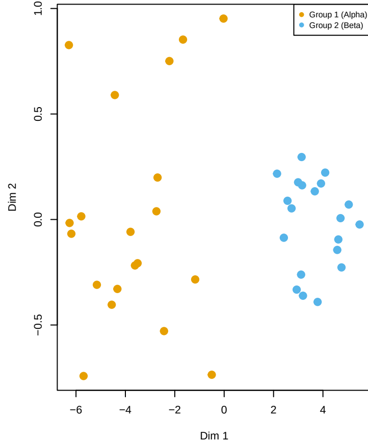
MDS – AIRM (Model A)
