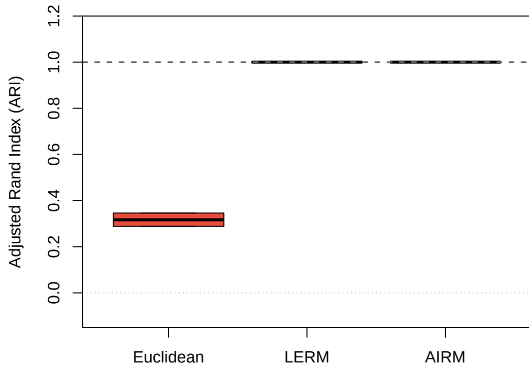
Model B – ARI Distribution
