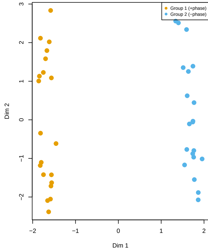
MDS – AIRM (Model B)
