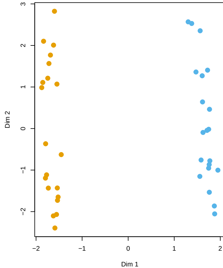
MDS – LERM (Model B)
