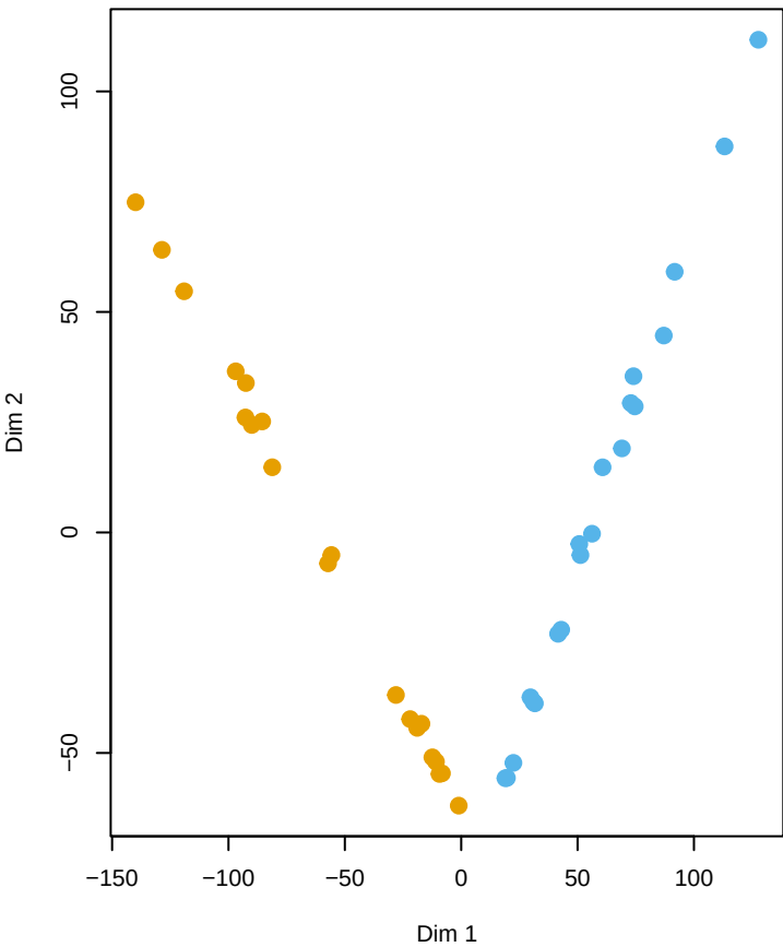
MDS – Euclidean (Model B)
