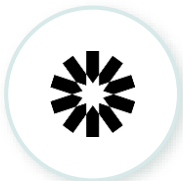
JWT
