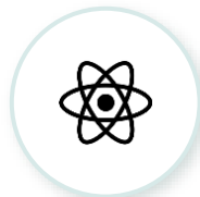
React 19
