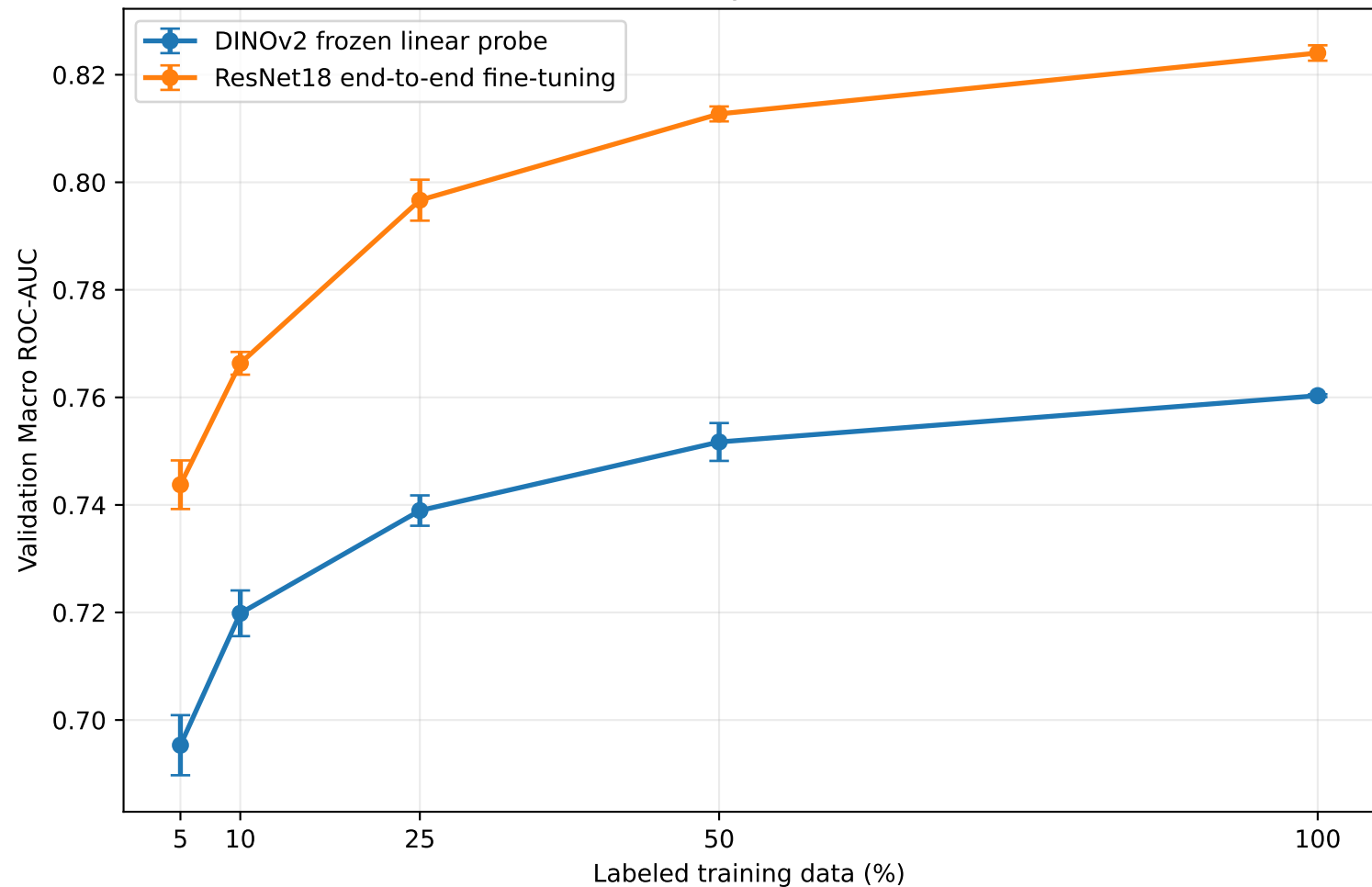
Label Efficiency on ChestMNIST
