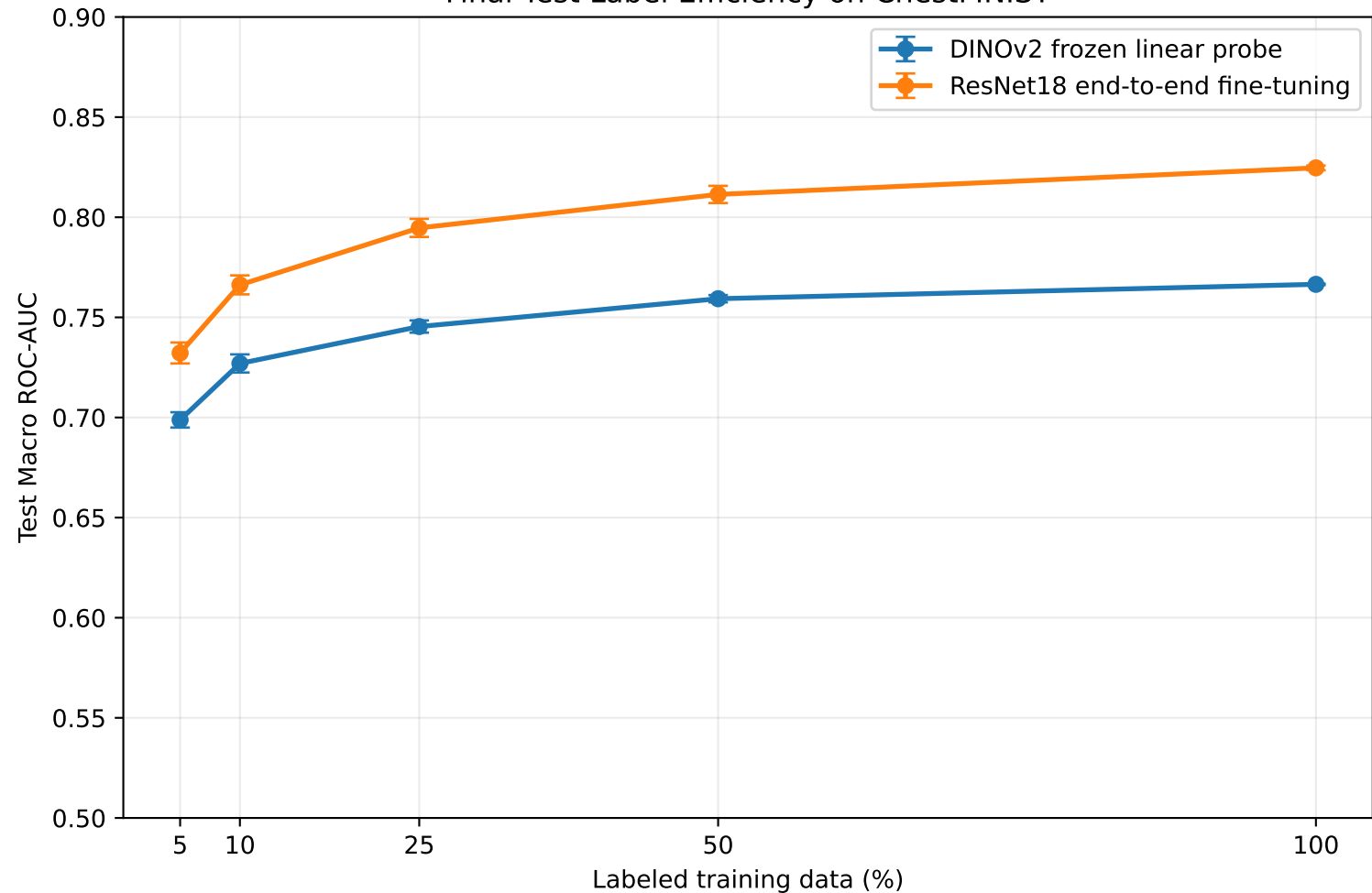
Final Test Label Efficiency on ChestMNIST
