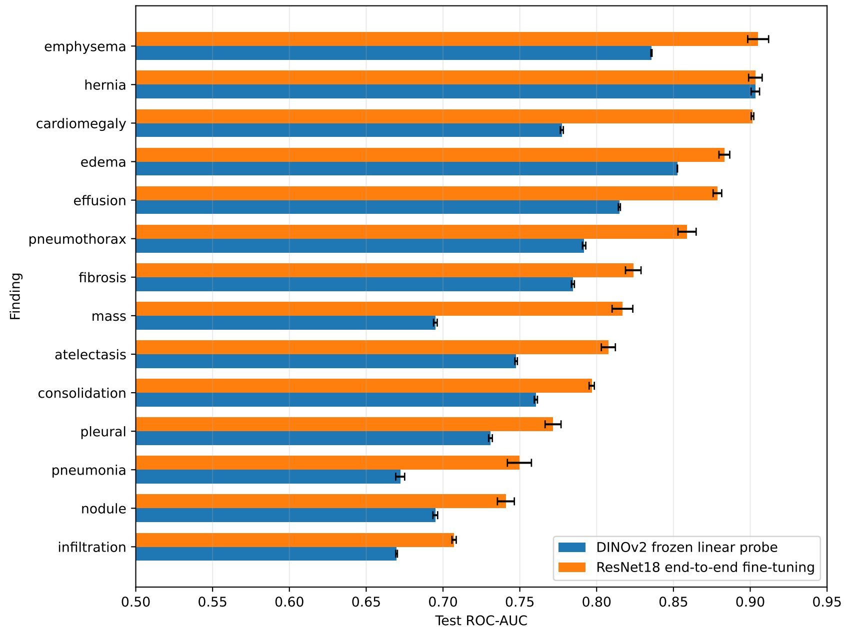
Final Test Per-Class Performance with 100% Labeled Data
