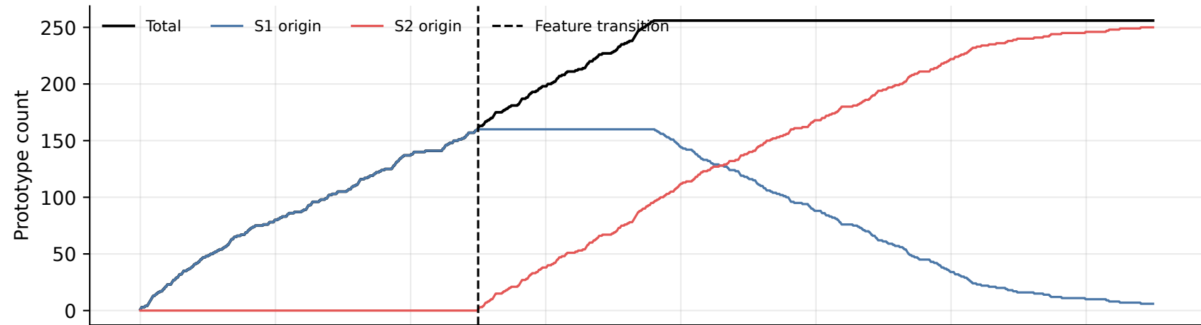
Prototype-bank evolution
