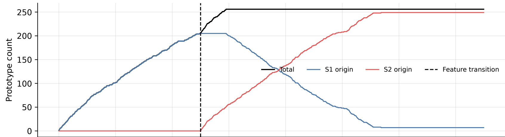
Prototype-bank evolution
