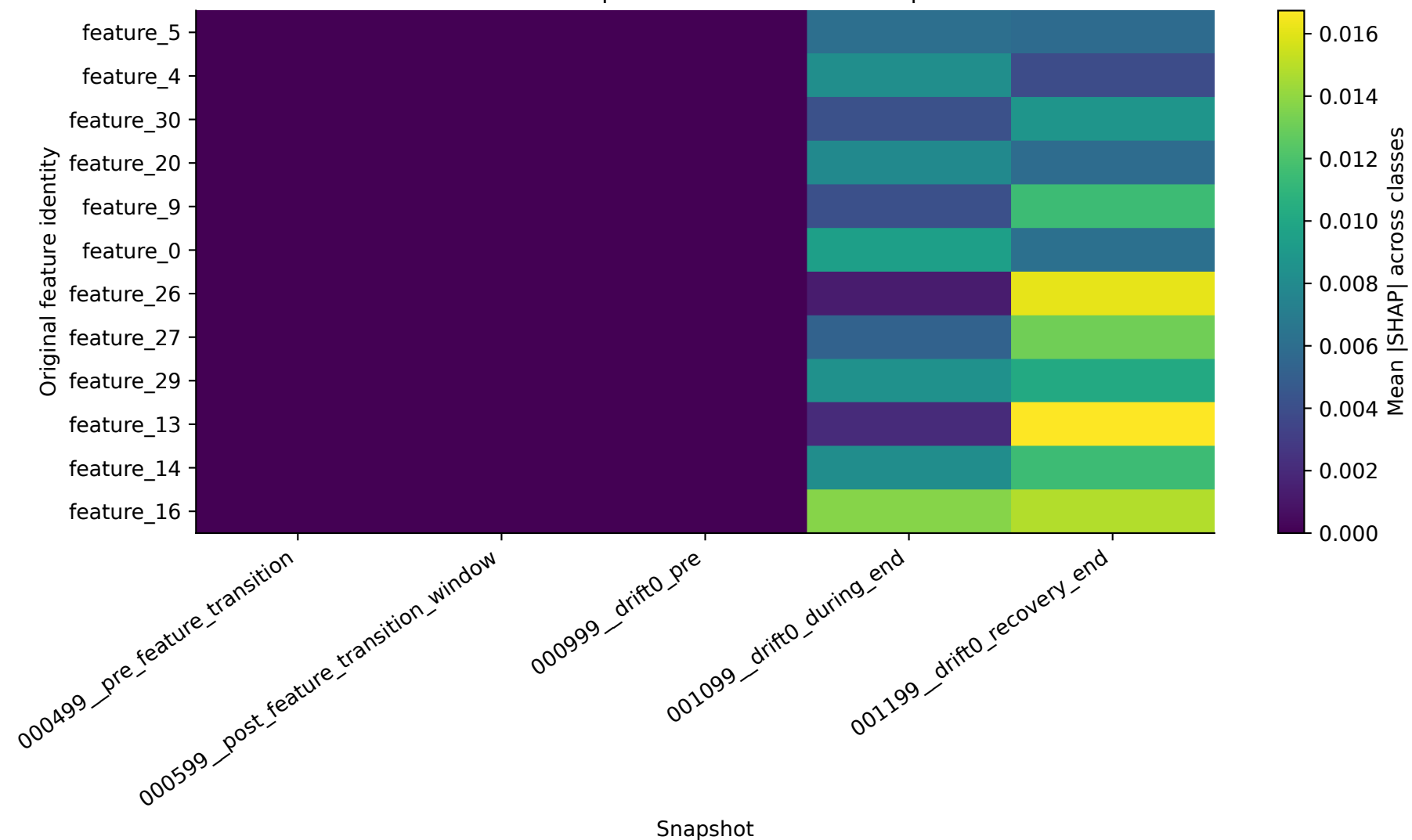
Global SHAP importance across online snapshots
