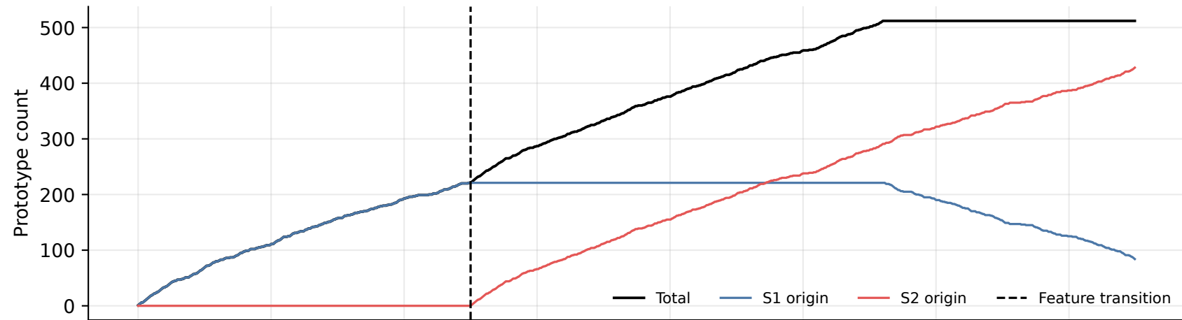
Prototype-bank evolution
