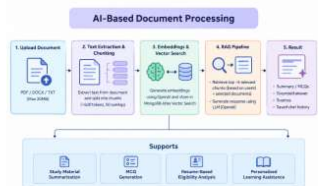
Fig. 2: AI-Based Document Processing
