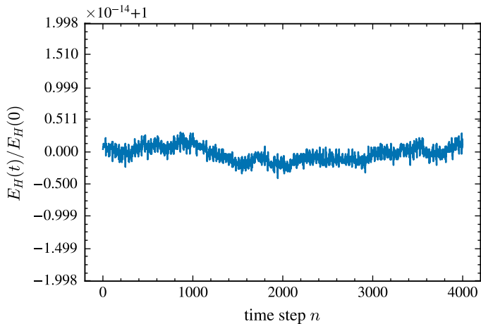
Discrete energy (symmetric Ventcel leapfrog)
