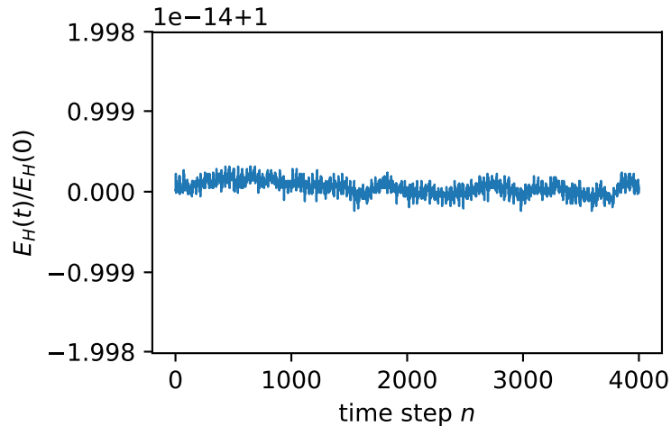
Discrete energy (symmetric Nitsche leapfrog)
