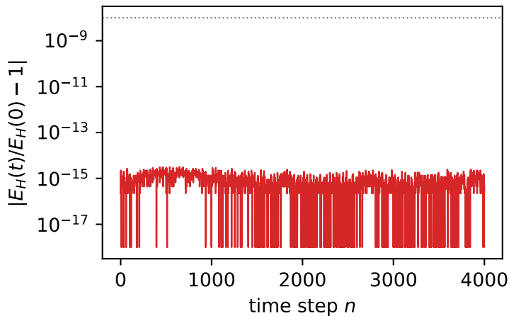
drift (max = 3.1e-15 , machine precision)
