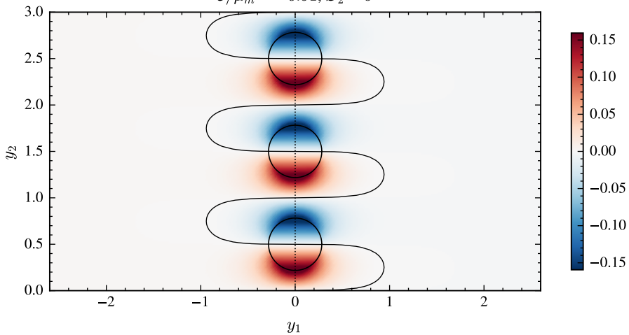
(b) tangential corrector Q^{(2)} \mathcal{C}/\mu_m = -0.91, \mathcal{B}_2 \approx 0
