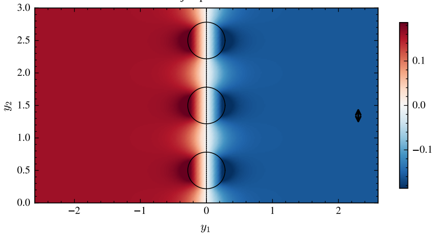
(a) normal corrector Q^{(1)} = U - y_1 far-field jump = \mathcal{B} = -0.31
