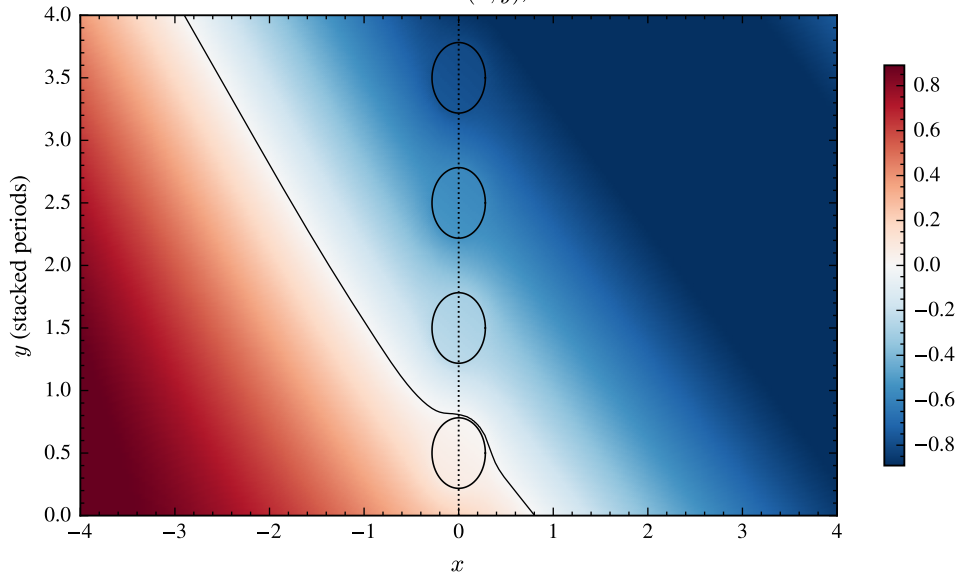
resolved 2D field \text{Re } U(x, y) , 45^\circ incidence
