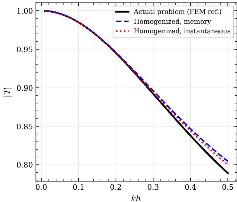
(b) Transmission coefficient |T|
