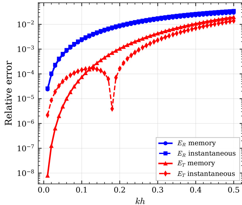
(c) Relative errors E_R, E_T
