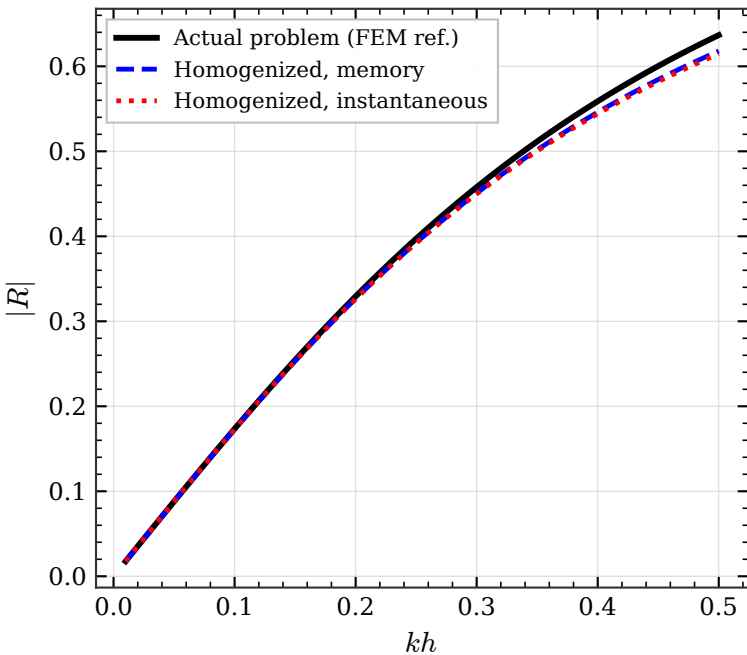
(a) Reflection coefficient |R|
