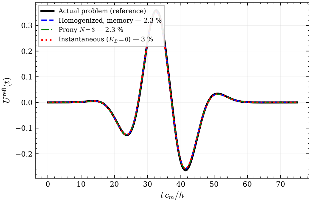
Weakly viscous matrix (test case): \omega\beta_m/\mu_m = 0.1
