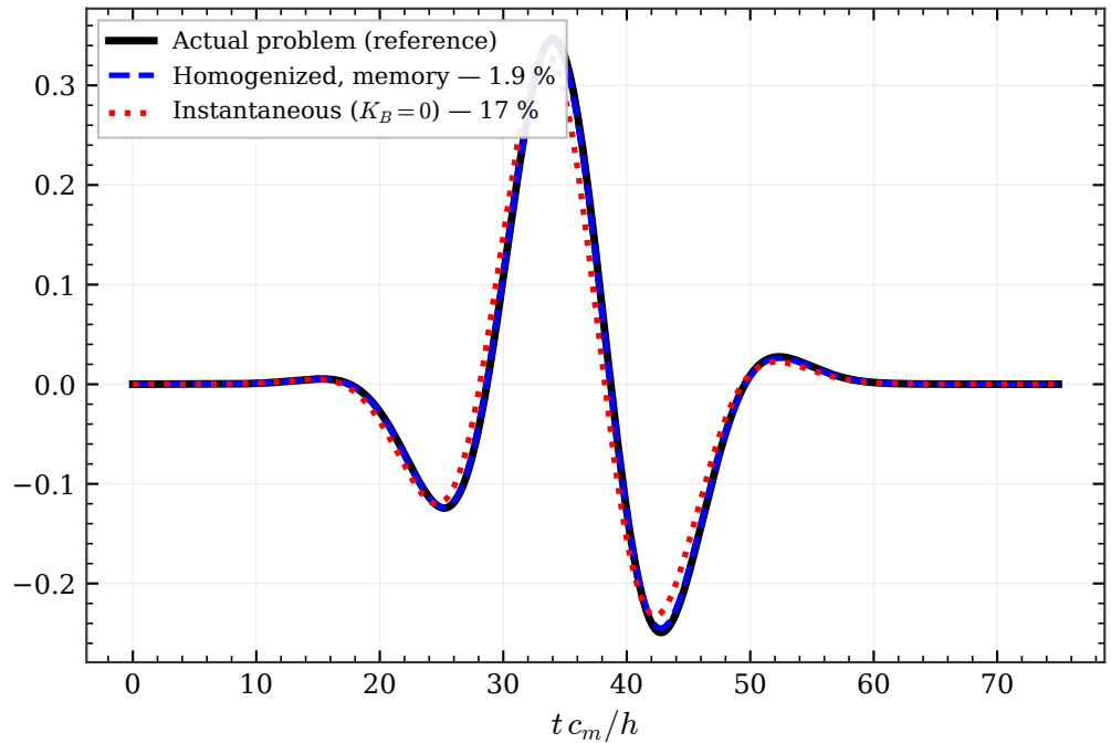
Dissipative matrix: \omega\beta_m/\mu_m = 3
