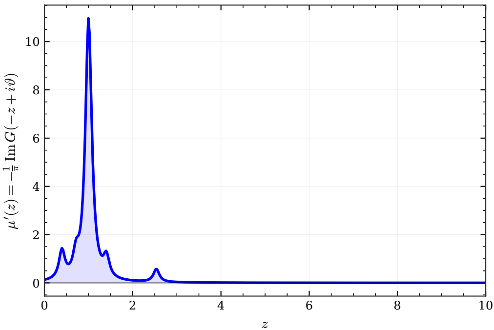
Stieltjes measure \mu' \geq 0
