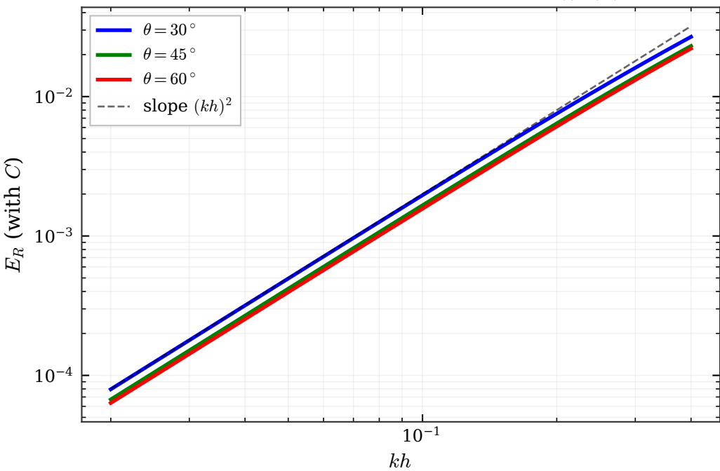
The complete model converges as \mathcal{O}((kh)^2)
