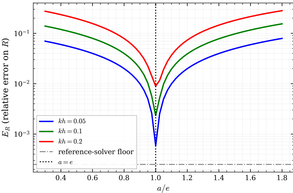
The error is minimal at a = e
