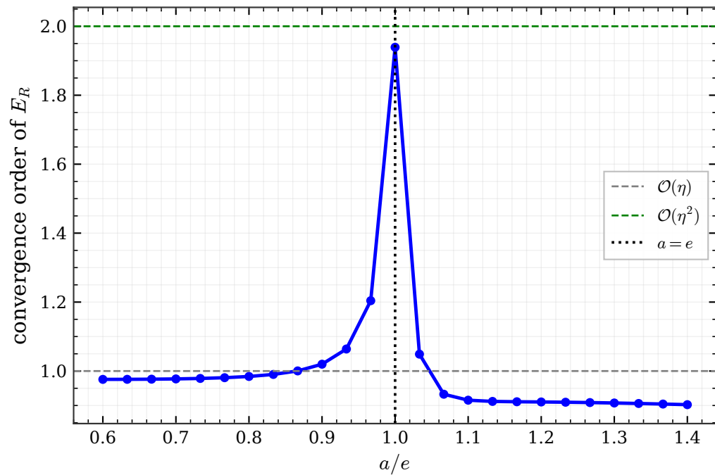
a = e is the only superconvergent choice
