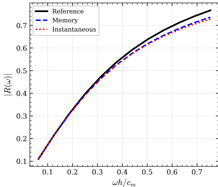
(b) Frequency-by-frequency reflection
