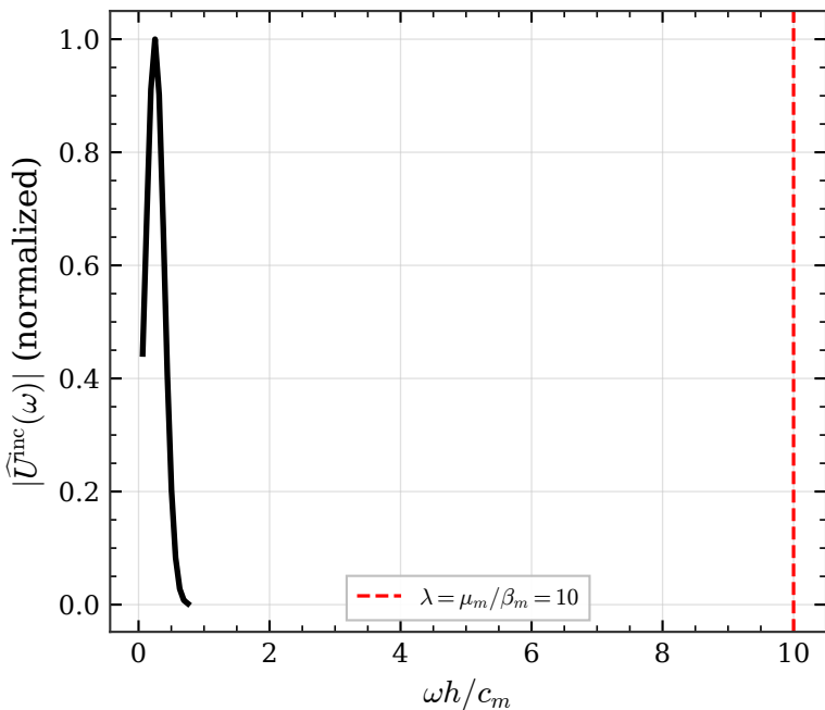
(a) Spectrum of the incident pulse
