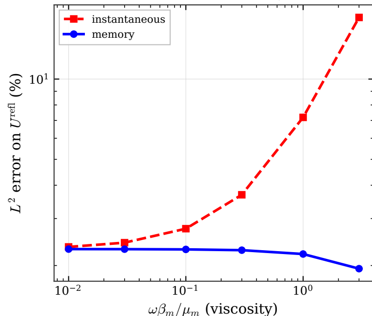
(c) Error vs viscosity
