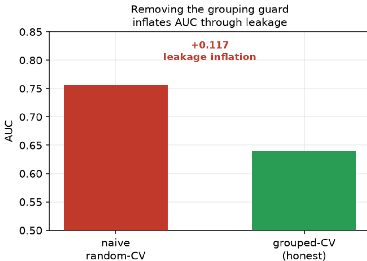
Figure 3: What the pre-registered guards caught. Removing shape-family grouping inflates AUC by +0.117; removing the effect-size gate lets an increment of +0.003 pass at p = 2 \times 10^{-24} on 55,000 networks.
