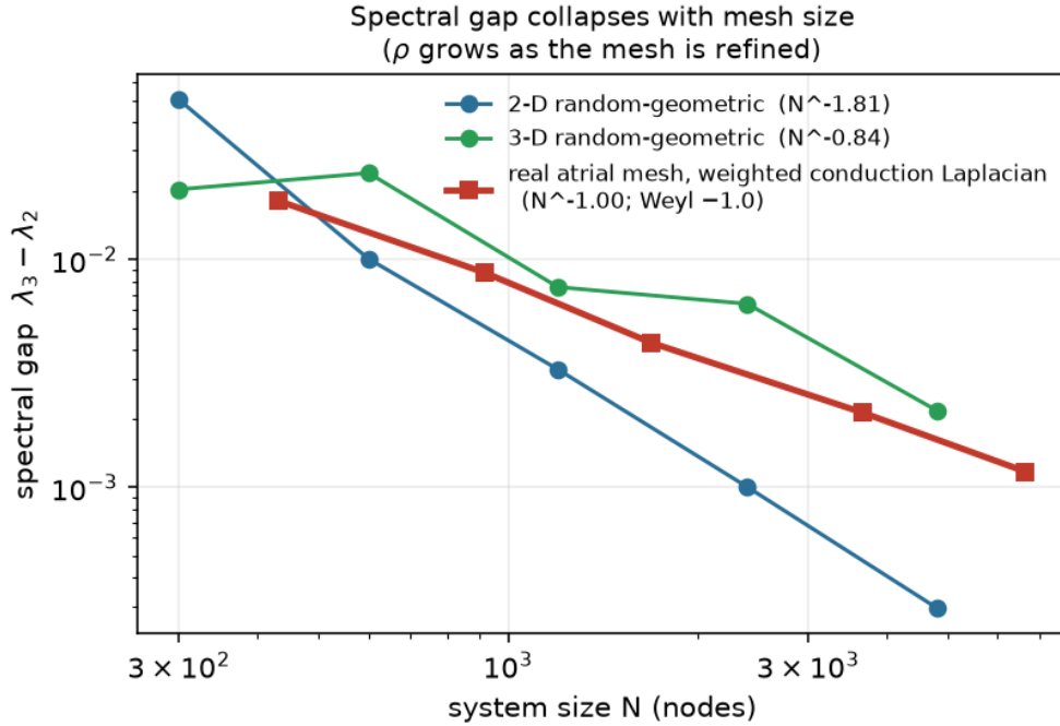
Figure 2: The estimator-validity boundary. The spectral gap collapses as the mesh is refined, at an exponent within 0.5% of the Weyl 2-manifold value, so \rho grows and the first-order estimator degrades more on a finer mesh of the same anatomy. The atrial curve is measured on the weighted conduction Laplacian the biomarker itself uses.
