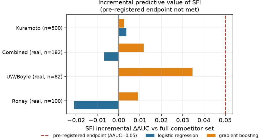
Figure 1: The predictive null. Adding the Spectral Fragility Index to the competitor set does not clear the pre-registered effect-size gate in any cohort; on the combined real cohort the bootstrap interval excludes the gate as well as containing zero.
