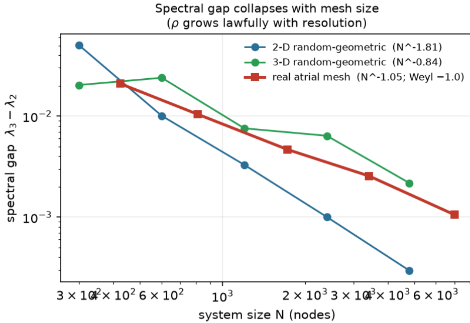
Figure 2: The gap collapses with mesh resolution, so the estimator degrades more , predictably, as the medium is meshed finer, the opposite of “more resolution helps.” Only the real atrial 2-manifold cleanly matches the Weyl exponent ( -1.05 vs. -1.0 ); the random-geometric exponents are reported as “at least as fast as Weyl,” not law confirmations, and use the unweighted combinatorial Laplacian.
