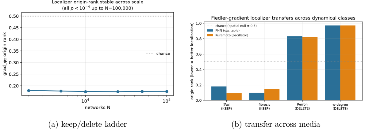
Figure 3: The weak-rank localization pattern replicates across excitable and oscillator dynamics. Three caveats apply: (i) the strict endpoint is null, so |V\varphi_2| is not a precise localizer; (ii) the substrate field co-localizes, and a controlled dissociation experiment shows why (in a diffusively-coupled medium the Fiedler bottleneck is the low-conduction lesion), so |V\varphi_2| matches, and does not beat, substrate imaging; (iii) the cardiac arm rests on only \sim 20 origins.
