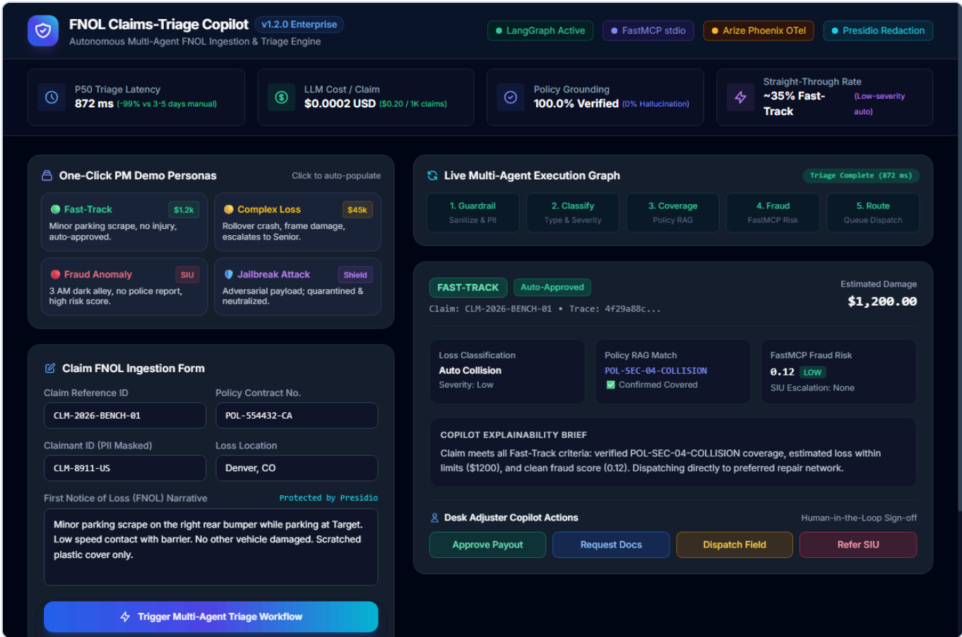
Figure 1: Live Web Screen Output. The 5 helpers light up in green, damage is calculated ($1,200), policy clause POL-SEC-04-COLLISION is verified, and the claim is Auto-Approved in 872 ms!
