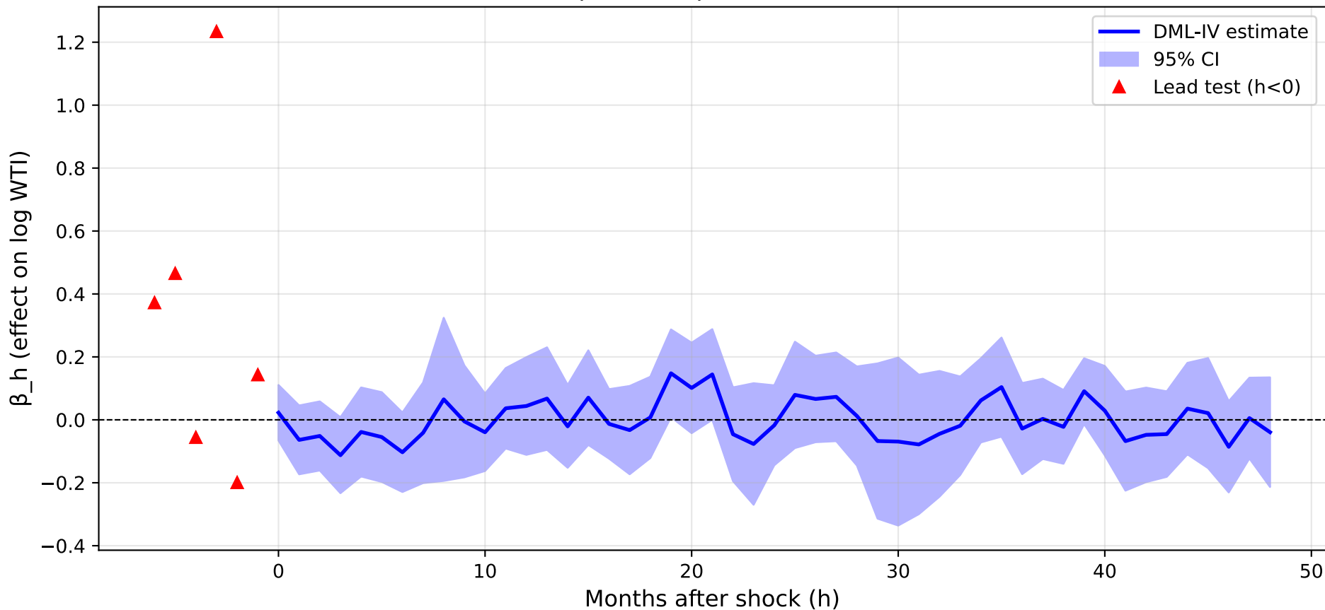
DoubleML-IV Impulse Response - Saadaoui Extension
