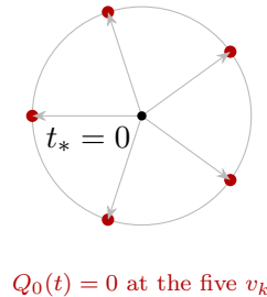
Figure 2: The explicit sextic calibration. The left star records which two roots collide at each event; the right pentagon records when the events occur. The LL map retains the right-hand schedule and forgets the left-hand gluing data.
