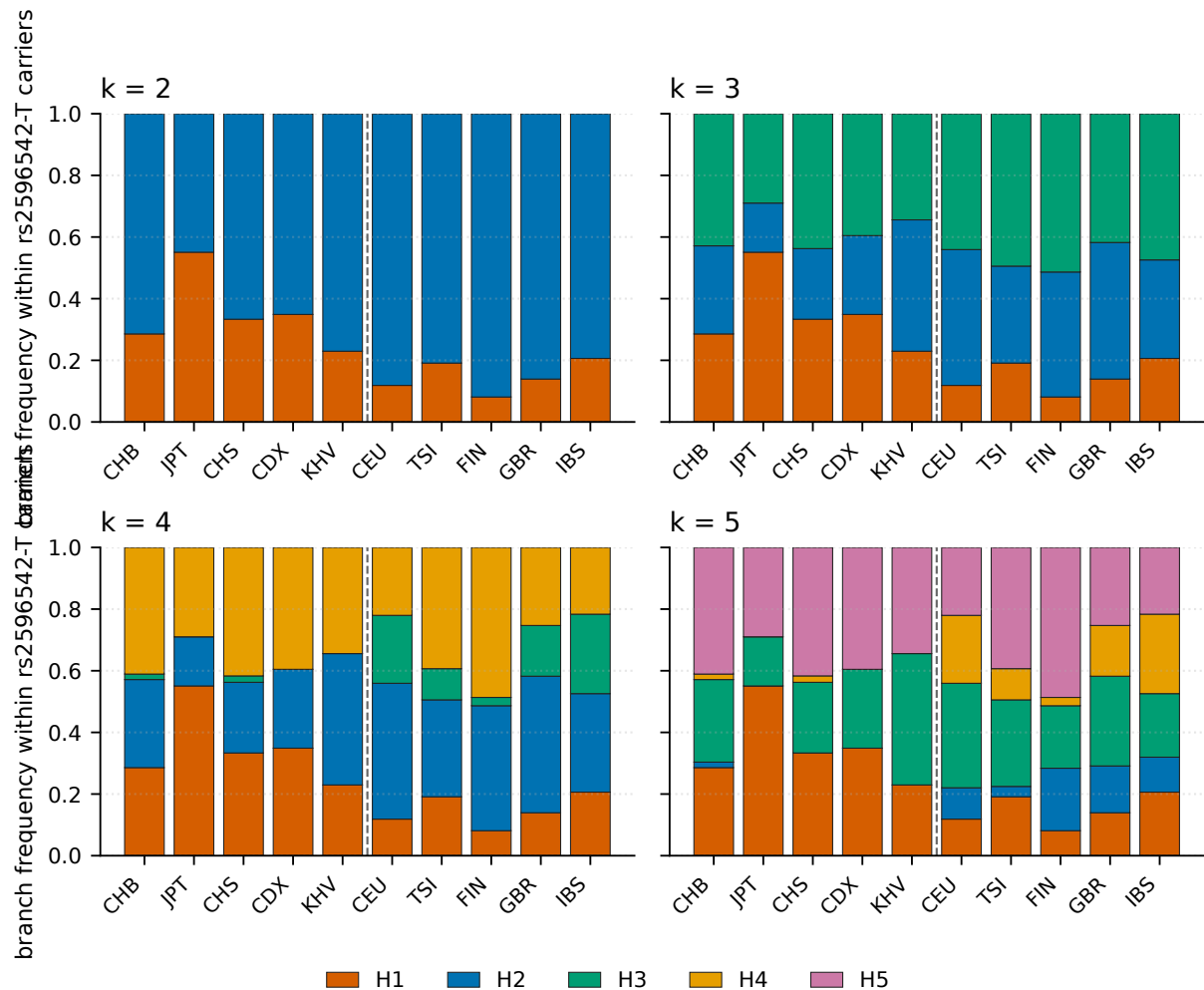
Figure 2. Branch composition by population — rs2596542-T anchor.
