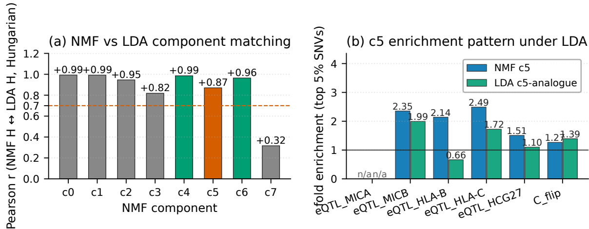
Supplementary Figure S1. NMF vs LDA decomposition on the same rs2596542-T carrier haplotype matrix ( k = 8 ).
