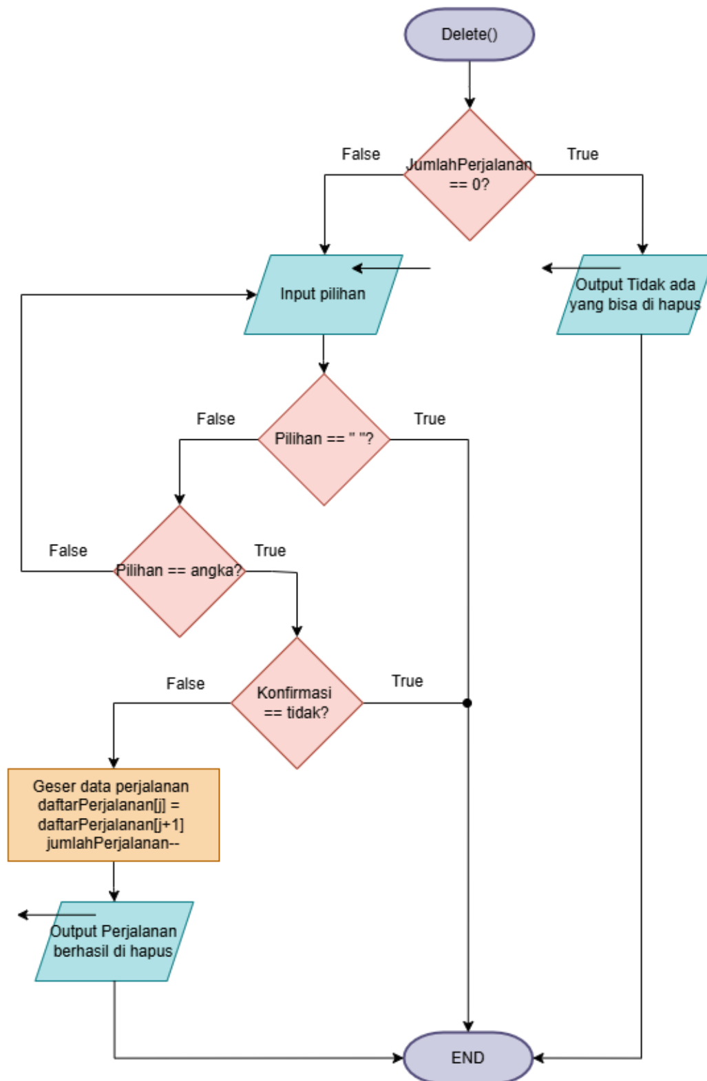
Gambar 1.7 Flowchart Hapus & Logout
