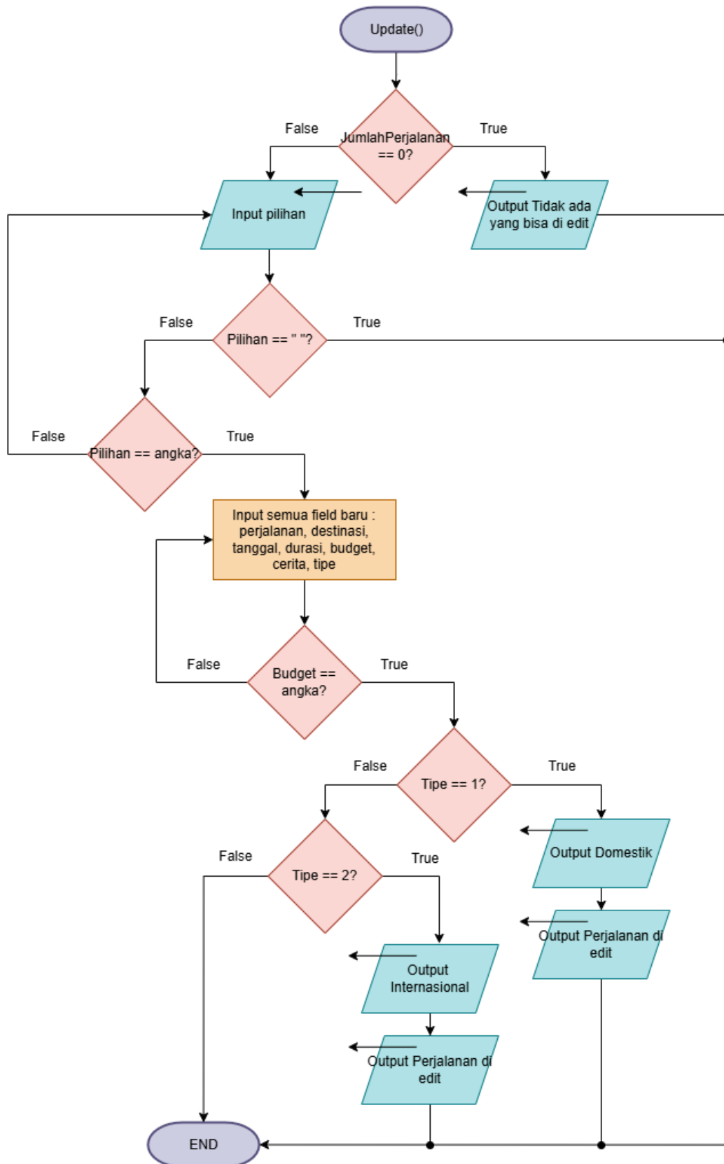
Gambar 1.6 Flowchart Update
