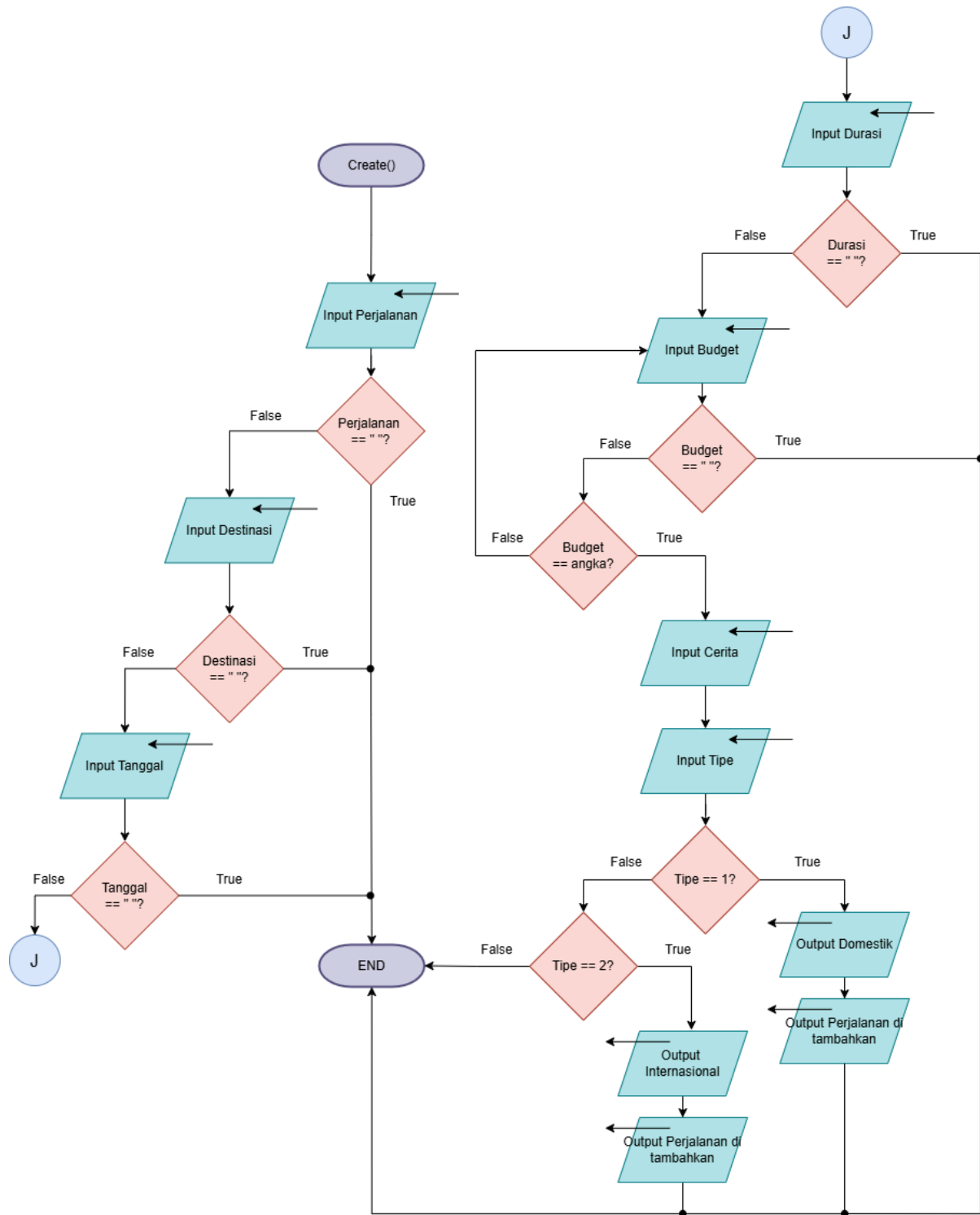
Gambar 1.5 Flowchart Create
