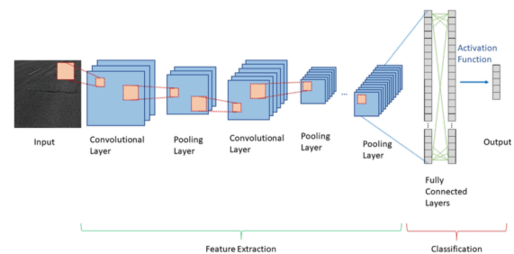
figure 3: architecture de CNN
