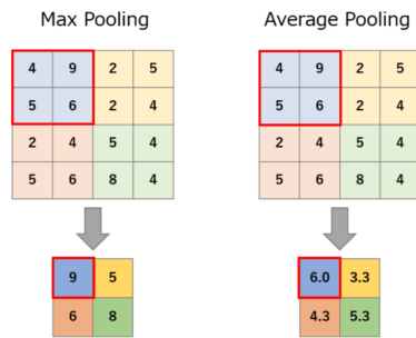
figure 5: couche de pooling
