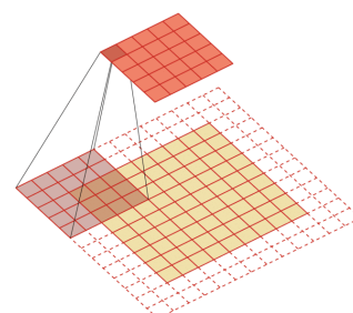
figure 4: couche convolutive
