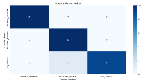
figure 8: matrice de confusion
