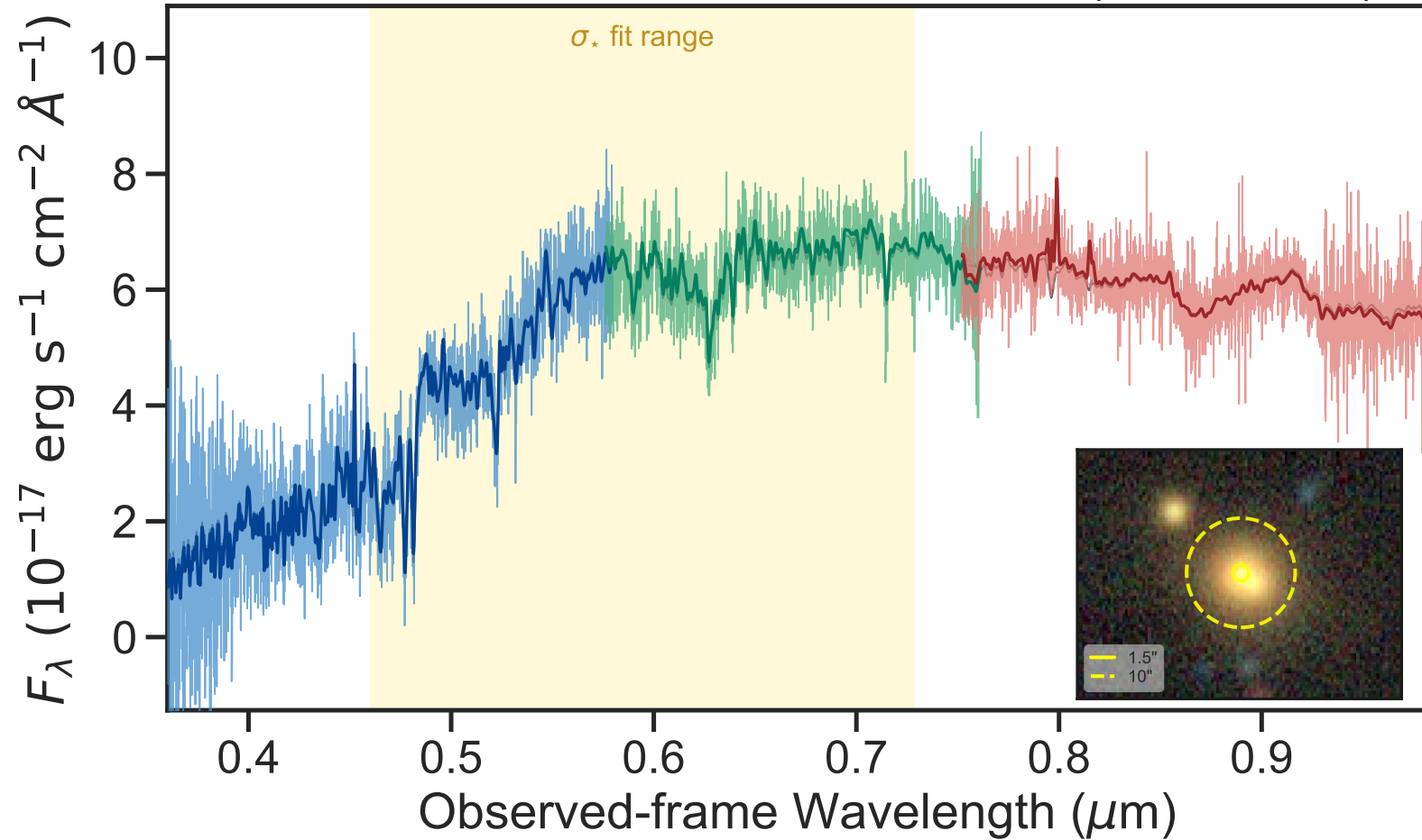
LRG TARGETID 39627496647296130 ( z = 0.2129 )
