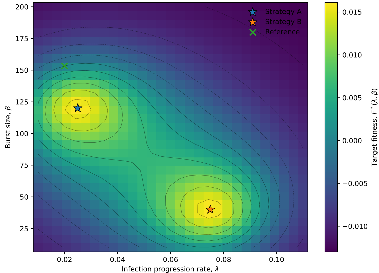
Stage 3: prescribed target fitness surface
