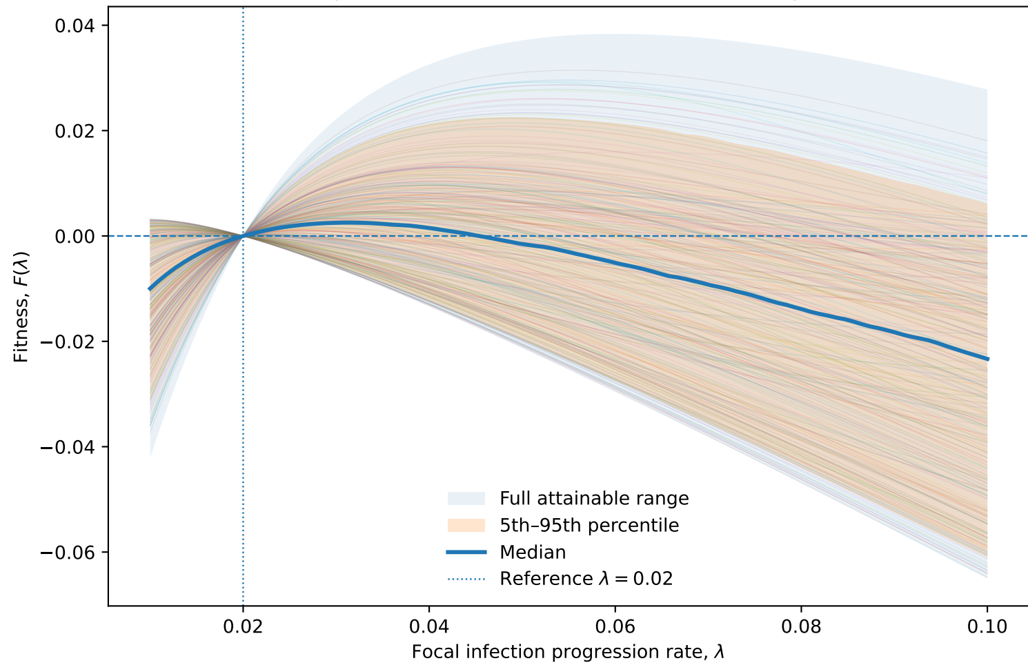
Experiment 0: attainable 1D fitness landscapes
