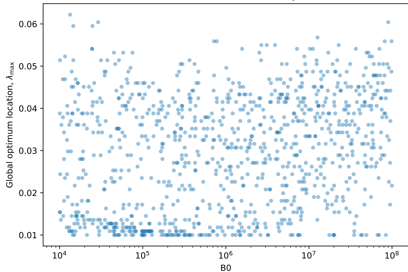
B0 versus location of the fitness optimum
